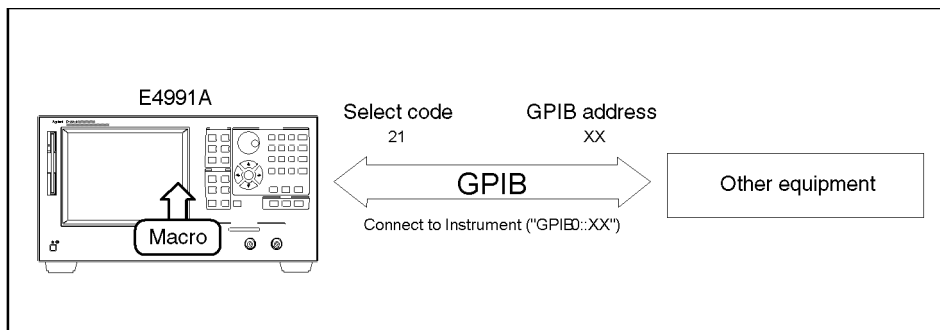
Structure example of GPIB remote control system
