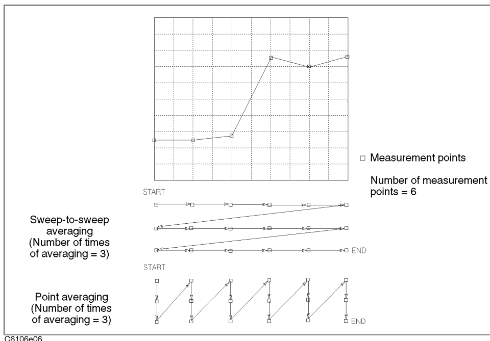
Sweep Averaging and Point Averaging
